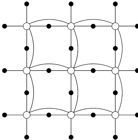
Fig. 1. Two-dimensional lattice (with L=3 ). The white circles are sites in \Lambda_o and the black dots are sites in \Lambda' . Electrons at a site can hop to another site if this site is connected to the original site with a line or a curve.
